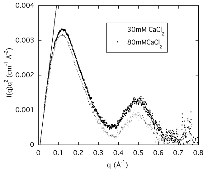
FIGURE 5 Kratky plot of the SAXS signals from a 3 wt % DNA solution containing 100 mM NaCl and either 30 mM \text{CaCl}_2 or 80 mM \text{CaCl}_2 at 14.900 keV. The straight line shown is the least-squares fit through the low q -data points, as described by Eq. 5.
