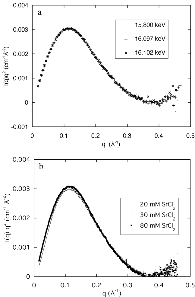
FIGURE 4 (a) Kratky plot of the SAXS signals from a 3 wt % DNA solution containing 100 mM NaCl and 80 mM \text{SrCl}_2 at 15.800 keV ( \blacksquare ), 16.097 keV (+), and 16.102 keV ( \times ). For clarity, only 10% of the data from each spectrum are plotted; (b) Kratky plot of the SAXS signals at 15.800 keV from three DNA solutions (3 wt %) containing 100 mM NaCl and 20 mM, 30 mM, and 80 mM \text{SrCl}_2 respectively.
