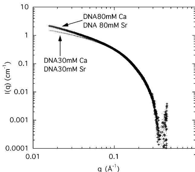
FIGURE 3 SAXS scattering from a 3 wt % DNA aqueous solution containing 100 mM NaCl and 30 mM \text{CaCl}_2 or 30 mM \text{SrCl}_2 (lower curves), and 80 mM \text{CaCl}_2 or 80 mM \text{SrCl}_2 (upper curves).
