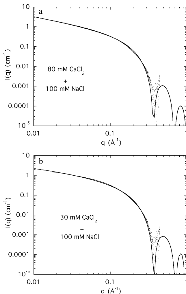
FIGURE 8 (a) SAXS spectrum from a 3% DNA solution in water containing 100 mM NaCl and 80 mM \text{CaCl}_2 . The fit is Eq. 6, with \chi = 5.9 \text{ cm}^{-1} , r_1 = 10.0 \text{ \AA} , r_2 = 13.8 \text{ \AA} , h = 0.25 , and L = 200 \text{ \AA} ; (b) SAXS spectrum from a 3% DNA solution in water containing 100 mM NaCl and 30 mM \text{CaCl}_2 . The parameters to the fit of Eq. 6 are \chi = 2.7 \text{ cm}^{-1} , r_1 = 10.0 \text{ \AA} , r_2 = 15.5 \text{ \AA} , h = 0.24 , and L = 90 \text{ \AA} .
