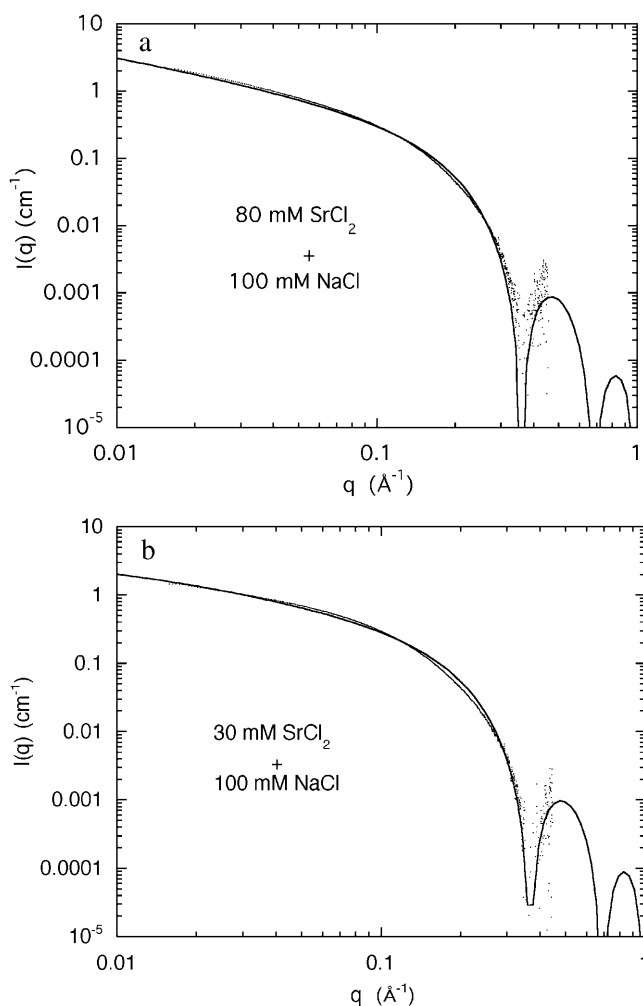
FIGURE 7 (a) SAXS spectrum from a 3% DNA solution containing an aqueous solution of 100 mM NaCl and 80 mM \text{SrCl}_2 . The fit is Eq. 6, with \chi = 4.3 \text{ cm}^{-1} , r_1 = 10.0 \text{ \AA} , r_2 = 13.8 \text{ \AA} , h = 0.40 , and L = 200 \text{ \AA} ; (b) SAXS spectrum from a 3% DNA solution containing an aqueous solution of 100 mM NaCl and 30 mM \text{SrCl}_2 . The parameters to the fit of Eq. 6 are I(0) = 2.4 \text{ cm}^{-1} , r_1 = 10.0 \text{ \AA} , r_2 = 13.8 \text{ \AA} , h = 0.265 , and L = 90 \text{ \AA} .
