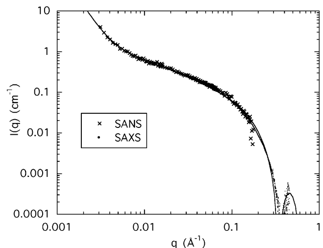
FIGURE 6 Normalized curves from SAXS at 15.8 keV and SANS for a 3% DNA solution in water containing 100 mM NaCl and 80 mM \text{SrCl}_2 . The SAXS data are converted to SANS contrast by multiplying the intensities by (\Delta\rho/r_0 K_p)^2 = 0.187 , corresponding to Model 1. The continuous line is Eq. 4 where L = 200 \text{ Å} , r = 11.1 \text{ Å} , and I(0) = 1.76 \text{ cm}^{-1} .
