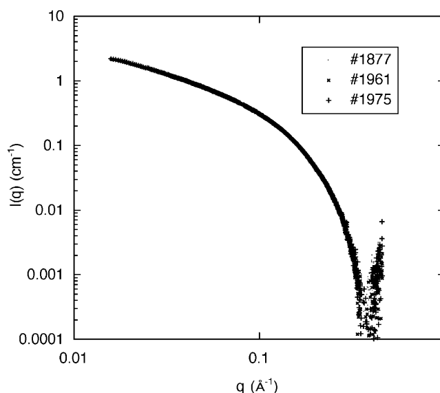
FIGURE 1 Scattering intensity at E = 15.8 keV from a 3 wt % DNA solution containing 80 mM strontium chloride, in three successive exposures of 50 s at the same position in the sample. In this q -range, the responses are indistinguishable.
