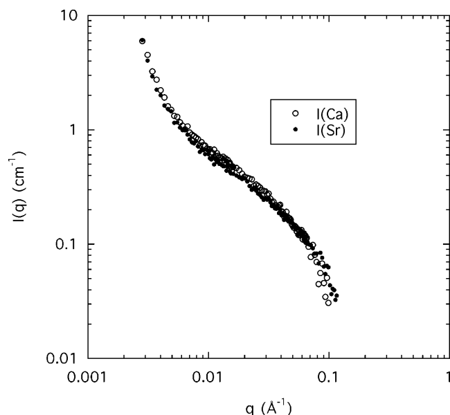
FIGURE 2 SANS response from a 3 wt % DNA solution containing 100 mM NaCl and 80 mM \text{CaCl}_2 (open symbols) or 80 mM \text{SrCl}_2 (solid symbols) in a 8% \text{D}_2\text{O} /92% \text{H}_2\text{O} mixture.
